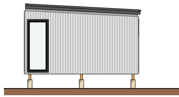
E-04 West Elevation Scale 1:100
