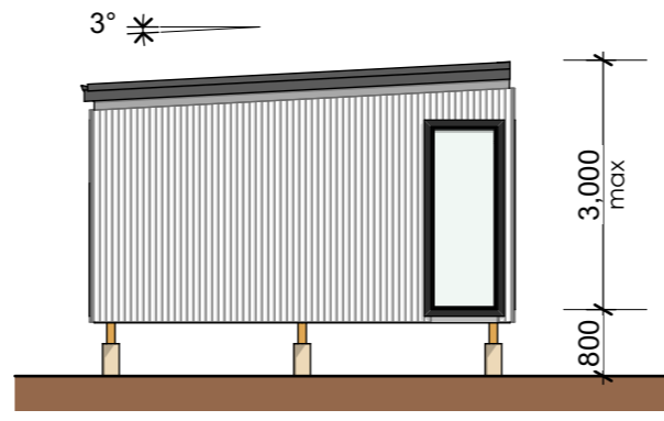
E-02 East Elevation Scale 1:100
