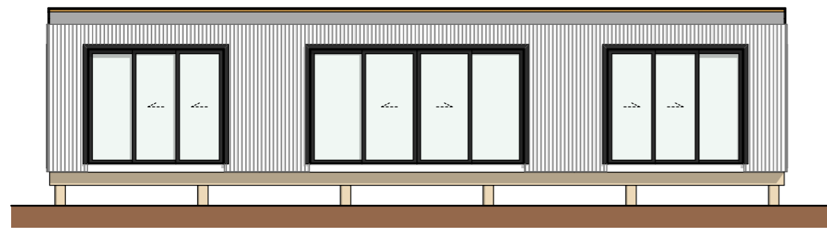
E-01 North Elevation Scale 1:100
