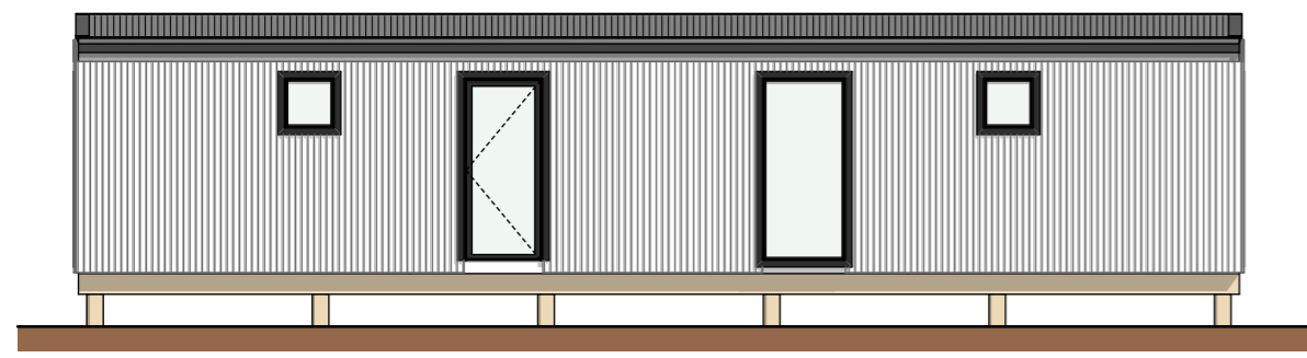
E-03 South Elevation Scale 1:100
