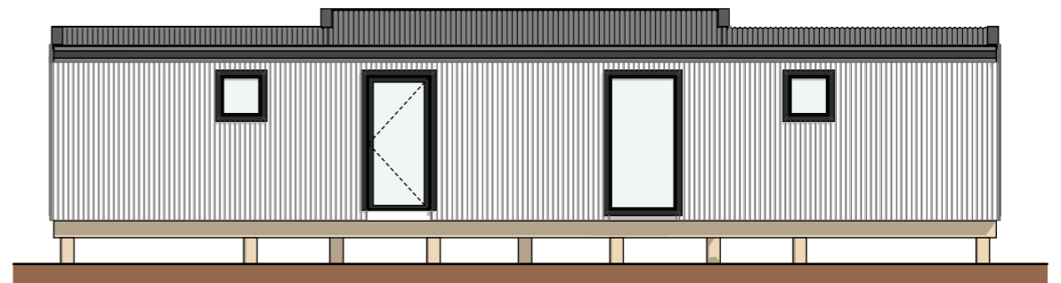
E-03 South Elevation
