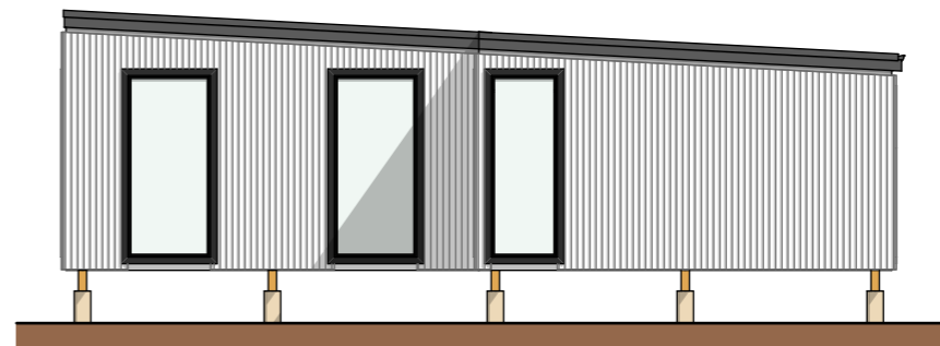
E-04 West Elevation
