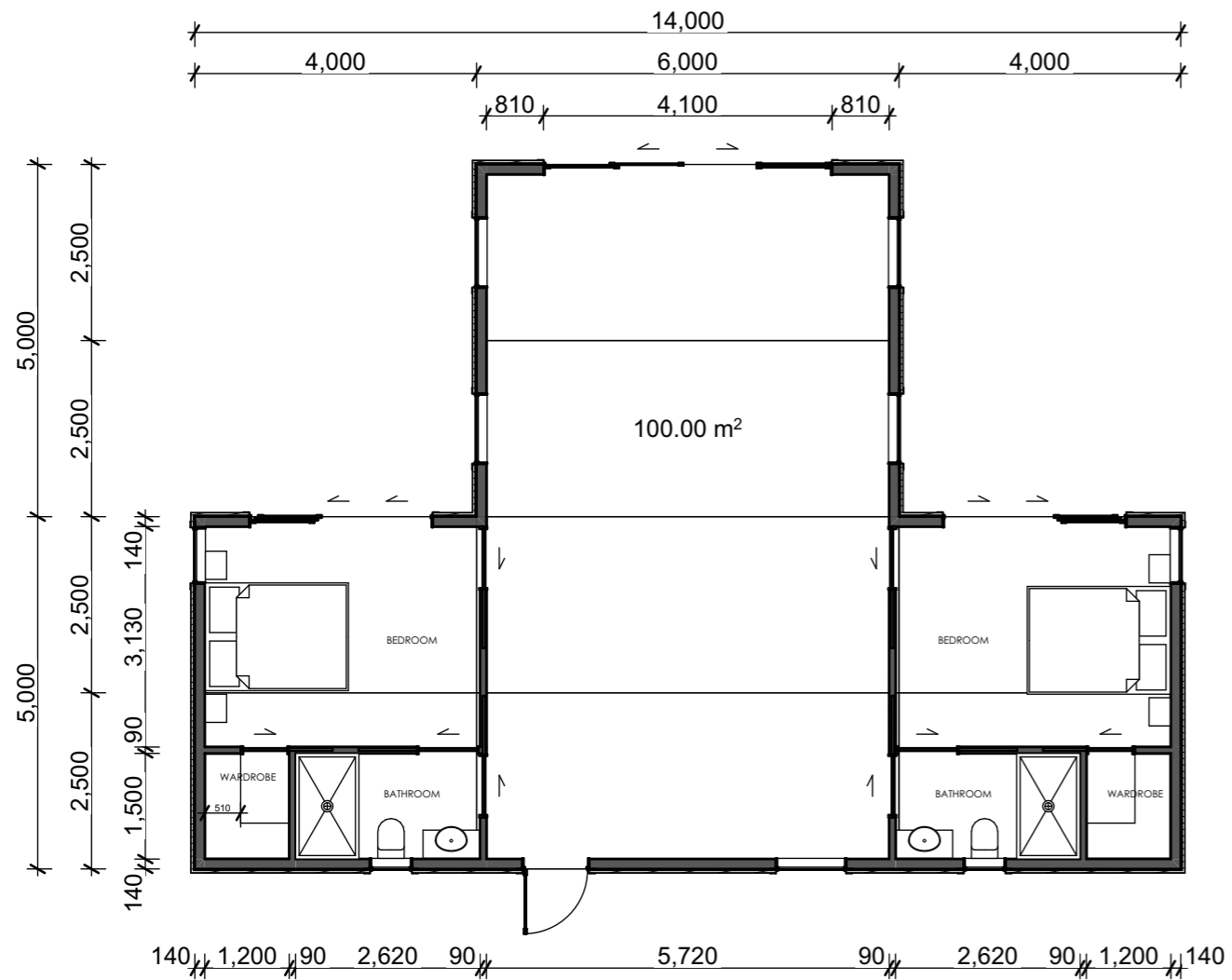
1 Floor Plan Scale 1:100
