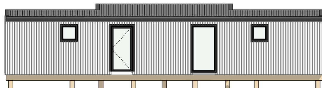
4 South Elevation Scale 1:100
