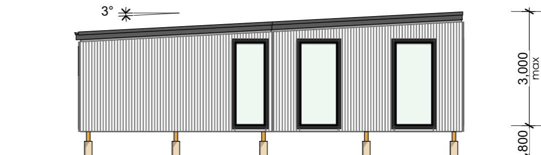
3 East Elevation Scale 1:100
