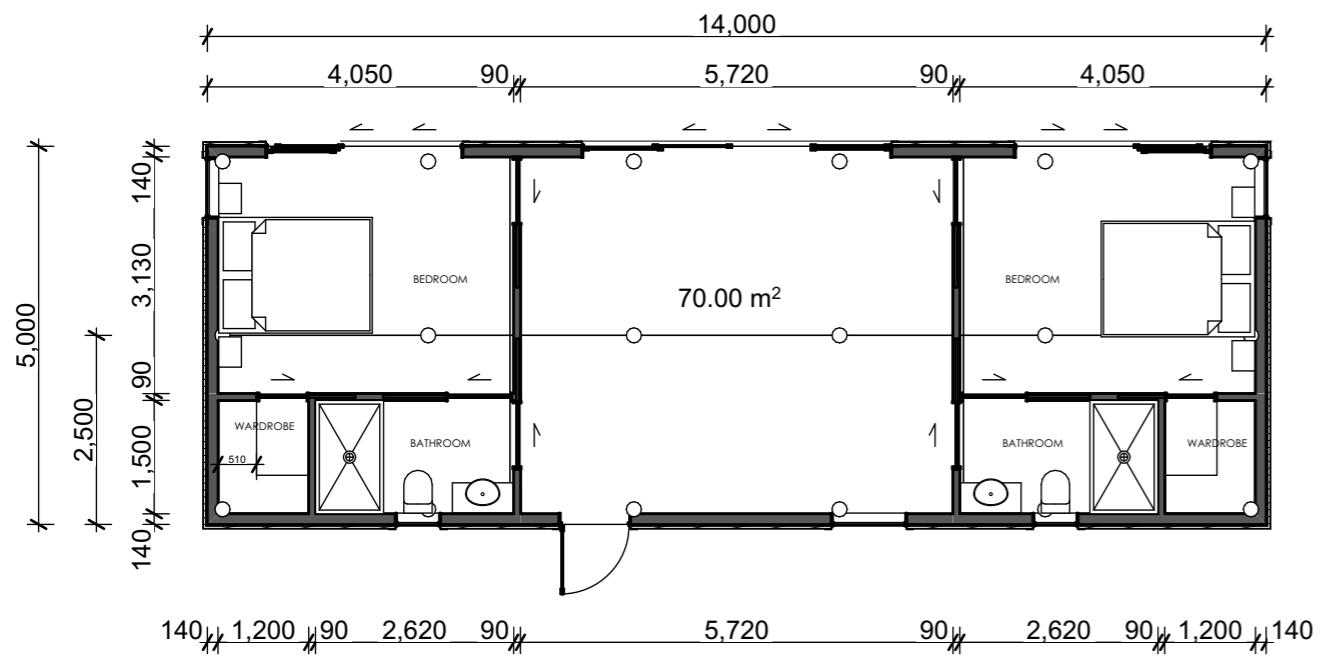
1 Floor Plan Scale 1:100
